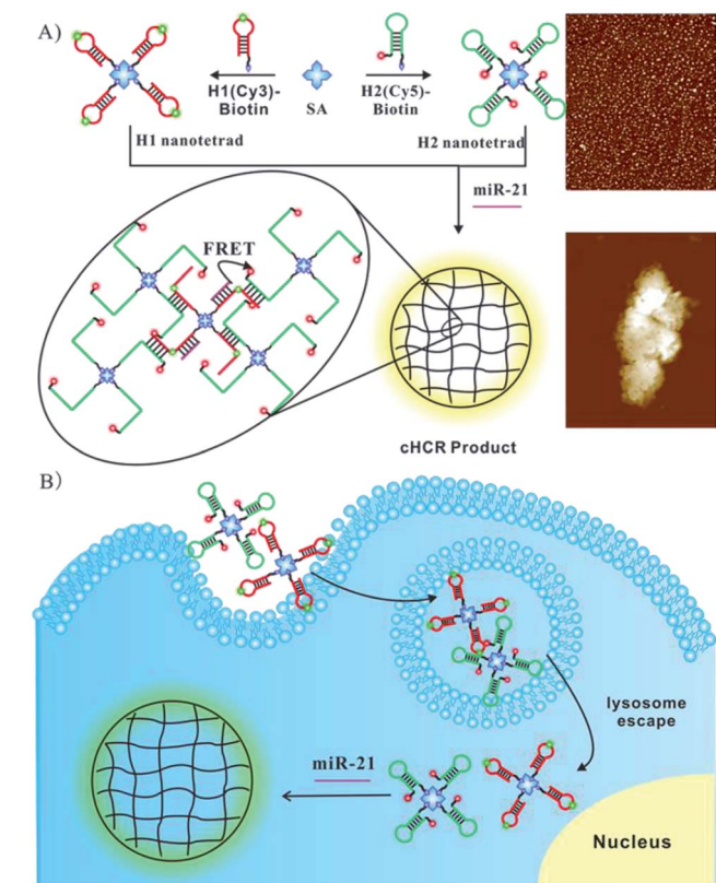
Scheme 1 Illustration of the (A) DNA tetrad enabled cHCR and (B) ultrasensitive intracellular miRNA imaging strategy.
