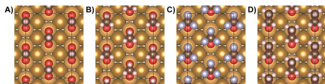
Fig. 4 Geometries used in calculations modeling densely-packed carboxylates: (A) formate, (B) acetate, (C) trifluoroacetate, (D) propenoate. A c(2 \times 2) unit cell was used for all cases, based on experimental measurements (STM and LEED).
