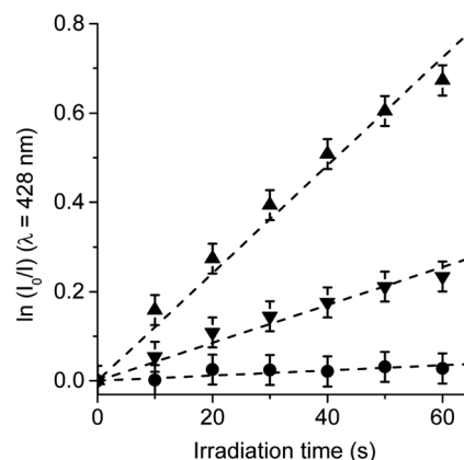
Fig. 9 Photooxidation of DMA in S. aureus cells ( \sim 10^6 CFU mL −1 ) incubated with 10 \mu M DMA for 30 min followed by a washing step and treated with 1 \mu M TCP-C 60 ( \blacktriangle ) or TCP-C 60 4+ ( \blacktriangledown ) for 30 min at 37 °C in dark. Control: S. aureus cells incubated with 10 \mu M DMA ( \bullet ); \lambda_{\text{irr}} = 455\text{--}800 nm.
