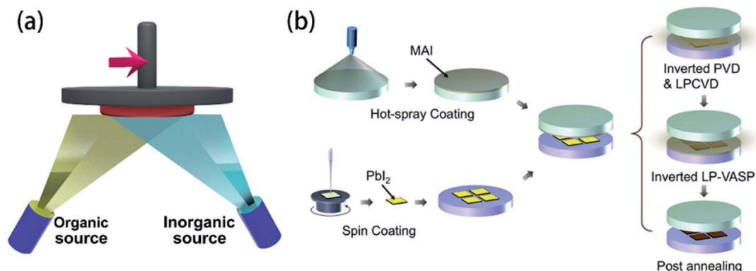
Fig. 10 (a) Schematic illustration of double source co-evaporation. (b) Schematic of vapor–solid reaction method. 32
