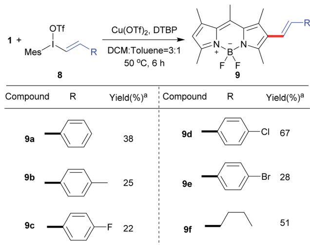
Scheme 5 Scope of the direct C–H vinylation of BODIPY 1 with different vinyl iodonium triflates. a Isolated yield.
