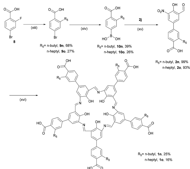
Scheme 3 Syntheses of campestarenes ( 1n and 1o ): (xiii) \text{R}_5\text{MgBr} , THF, \text{N}_2 , 17 h, then \text{HCl} ; (xiv) n -BuLi, \text{B(O-}i\text{-Pr)}_3 , THF, -78^\circ\text{C} , 3 h, then \text{HCl} ; (xv) \text{Na}_2\text{CO}_3 , \text{Pd(PPh}_3)_4 , \text{DMF/H}_2\text{O} , 105^\circ\text{C} , 6 h; (xvi) \text{Na}_2\text{S}_2\text{O}_4 , \text{EtOH/H}_2\text{O} , reflux, 2 h.
