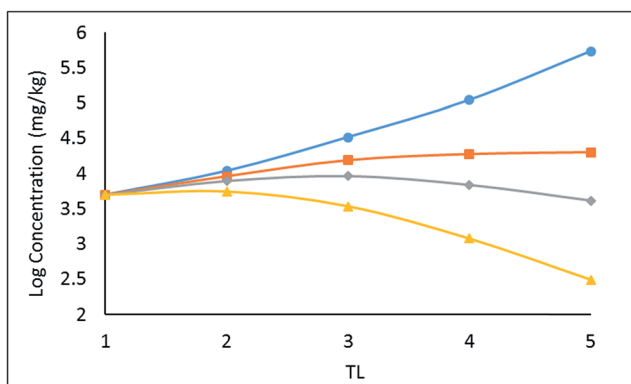
Fig. 3 Effect of biotransformation on \log C_{FW} in a food chain for selected values of k_M , specifically reading down: 0 (blue), 0.01 (orange), 0.02 (grey) and 0.05 (yellow) days -1 . The corresponding TMF_W values are 3.21, 1.42, 0.95, and 0.49.
