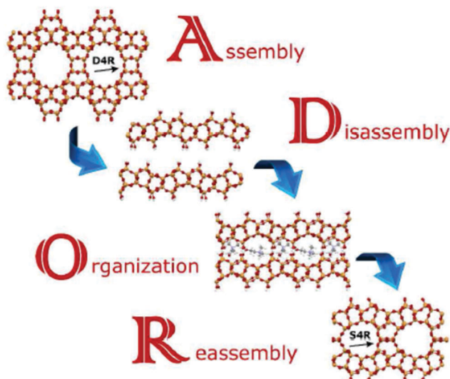
Fig. 8 Scheme of the ADOR process for transformation of the germanosilicate parent zeolites, Reproduced from ref. 232 with permission from the Royal Society of Chemistry, copyright 2017.
