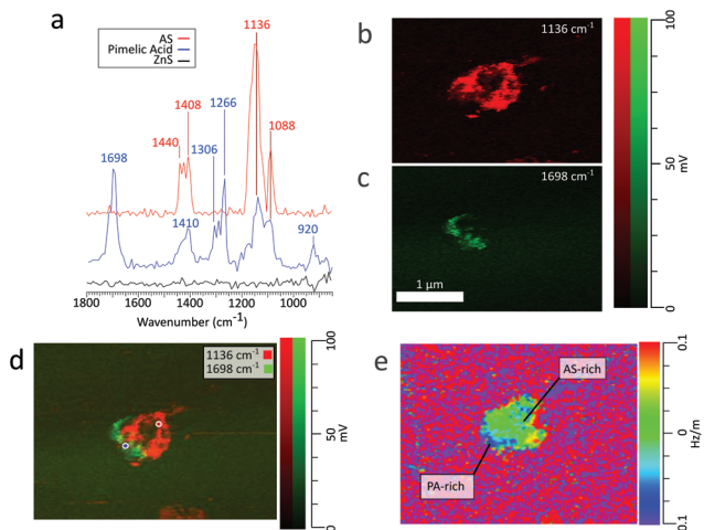
Fig. 6 (a) PTIR spectra obtained on a PA/AS particle for PA rich (blue) AS rich (red) and ZnS (black) regions at the corresponding locations marked in panel d. (b) Chemical image of the particle at 1136\text{ cm}^{-1} (c) chemical image of the particle at 1698\text{ cm}^{-1} (d) RGB overlay of chemical images in panels c and d. (e) Ratio image of the frequency map at 1136\text{ cm}^{-1} and height.
