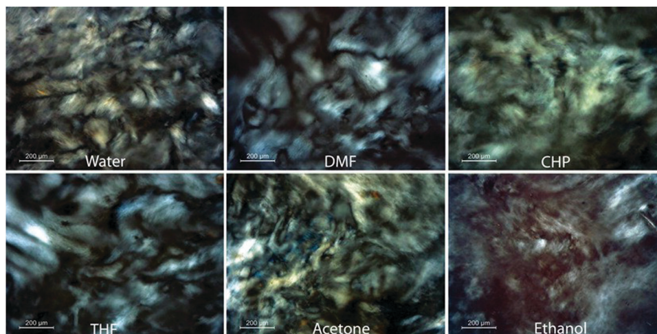
Fig. 5 Schlieren textures observed in dispersions of graphene oxide in a range of organic solvents under microscopy using crossed polarisers. Reproduced with permission from Jalili et al. , ACS Nano , 2013 78 (©2013 American Chemical Society).
