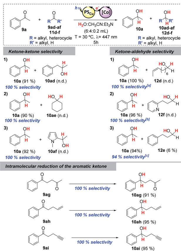
Scheme 3 Competitive photoreductions. Conditions: 1 (1 mol%), PS Cu (1.5 mol%), substrate A + B (16.5 mM, 1 : 1), in \text{H}_2\text{O} : \text{CH}_3\text{CN} : \text{Et}_3\text{N} (6 : 4 : 0.2 mL) irradiated (447 nm) for 5 h at 30 °C under \text{N}_2 . [a]35 [b]50 and [c]30 min reaction, respectively. The isolated products were identified and characterized using NMR Spectroscopy.
