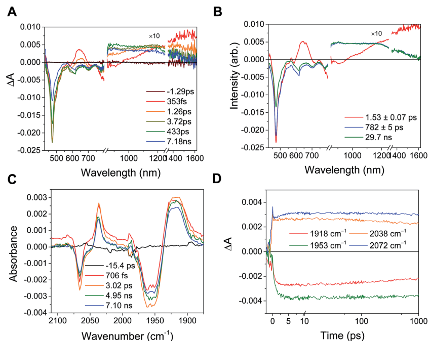
Fig. 10 (A) Transient absorption and (B) species-associated spectra for complex Phbpy-Re-PyPhNDI 1- (λ ex = 605 nm) showing biphasic back electron transfer kinetics. Kinetic traces and fits are shown in Fig. S7.† (C) fsIR spectra and (D) kinetic traces with fits for complex Phbpy-Re-PyPhNDI 1- (λ ex = 605 nm) showing monophasic back electron transfer kinetics. The instrument response is approximately 2 ps.
