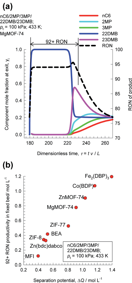
Fig. 9 (a) Transient breakthrough simulations for separation of equimolar n C 6 /2MP/3MP/22DMB/23DMB mixtures at 433 K and 100 kPa in fixed bed adsorber packed with MgMOF-74. Also shown is the RON of product gas at the outlet of fixed bed. (b) Comparison of 92+ RON productivity for operation at total pressure of 100 kPa, plotted as a function of the separation potential \Delta Q_{(22\text{DMB}+23\text{DMB})/(nC_6+2\text{MP}+3\text{MP})} , calculated from eqn (19) and IAST. All calculation details and structural information on the various MOFs are provided in the ESI.†
