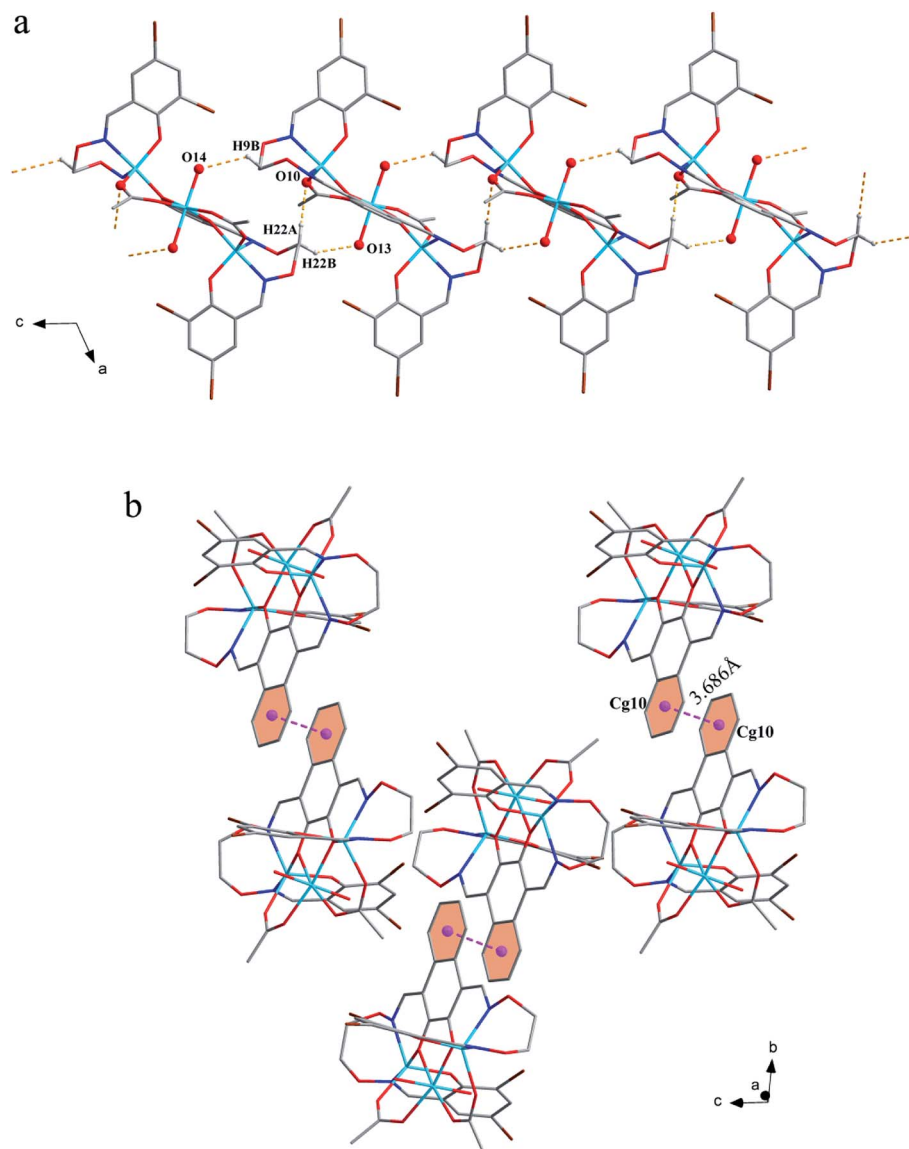
Fig. 7 (a) View of the 1D structure by intermolecular C–H...O interactions. (b) View of the 2D supramolecular layered by intermolecular \pi\cdots\pi interactions.
