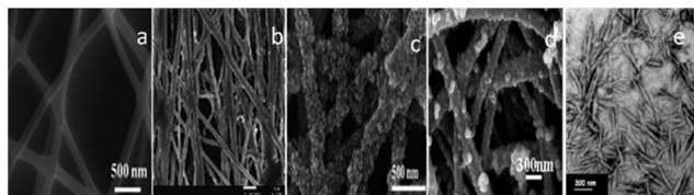
Fig. 1 SEM images of various types of CNF synthesized from cotton (a) natural electrospun CNF 56 (b) aligned CNF (scale bar 1 \mu m) 54 (c): CdS functionalized CNF 33 (d): CeO 2 functionalized CNF 56 (e): CNF prepared by acid hydrolysis 52 (adopted with permission).
