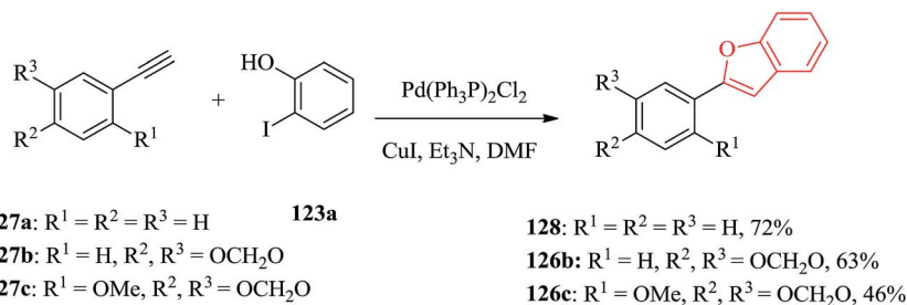
Scheme 30 Synthesis of arylbenzofurans 128 , 126b and 126c .
