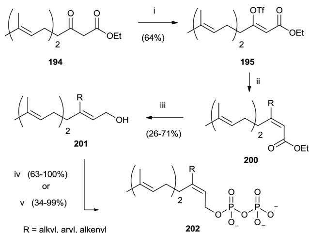
Scheme 35 Reagents and conditions: (i) (\text{Me}_3\text{Si})_2\text{NK} , \text{THF} , \text{PhN}(\text{SO}_2\text{CF}_3)_2 . (ii) \text{RMgX} , \text{CuCN} , ether. (iii) DIBALH, toluene. (iv) a: \text{NBS} , \text{CH}_2\text{Cl}_2 , \text{Me}_2\text{S} ; b: (\text{Bu}_4\text{N})_3\text{HP}_2\text{O}_7 , \text{CH}_3\text{CN} .
