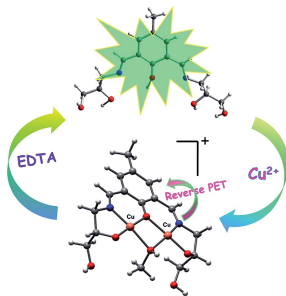
Scheme 2 Schematic illustration of proposed mechanism for the fluorescence changes of chemosensor ( H 5 dpm ) upon addition of \text{Cu}^{2+} .
