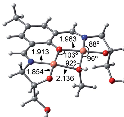
Fig. 7 BP86-D3/def2-TZVP optimized structure of [Cu_2(H_5dpm)MeOH]^+ complex. Distances are in Å.
