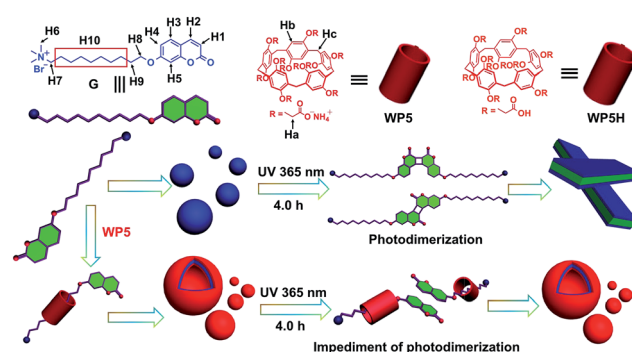
Scheme 1 Schematic representation of the hindrance of photo-dimerization and the self-assembly process of G and WP5-DG in water.
