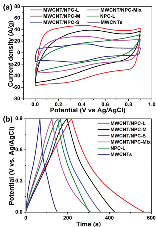
Fig. 7 (a) CV curves at a potential scan rate of 200 mV s -1 . (b) Charge-discharge curves at a current density of 1 A g -1 for MWCNT/NPC-S/M/L, MWCNT/NPC-Mix, NPC-L and MWCNTs.
