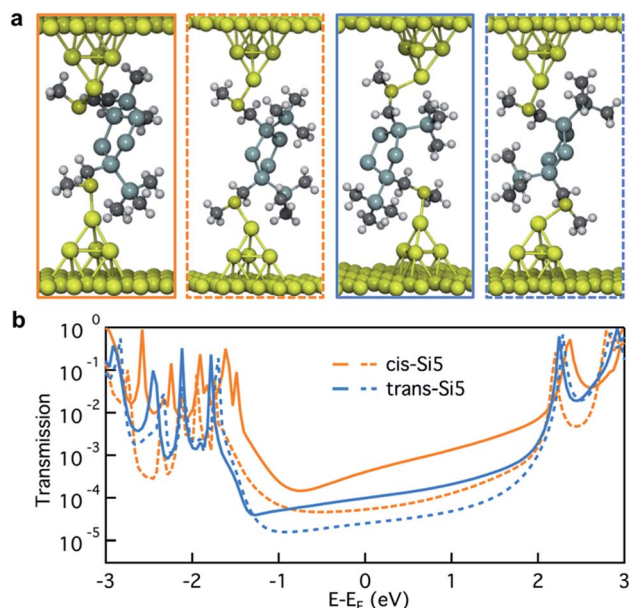
Fig. 4 (a) Geometries and (b) transmission curves of two example conformers of cis-Si5 and trans-Si5 (solid orange: cis-4-envelope-f2 ; dashed orange: cis-1-twist-e2 ; solid blue: trans-1-envelope-b4 ; dashed blue: trans-1-envelope-b3 ). Methyl groups on the ring have been removed for clarity.
