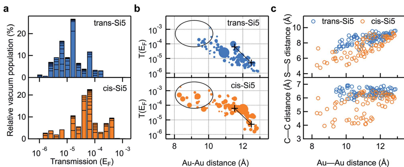
Fig. 5 (a) Logarithmically binned histogram of transmission at Fermi energy of the 91 trans-Si5 and 74 cis-Si5 conformers. The horizontal stack lines in the bars indicate the vacuum population of each conformer. The histogram is normalized to sum up to 100%. (b) Transmission at Fermi energy plotted against the Au-Au junction distance for each trans-Si5 and cis-Si5 conformer bridged between four-atom Au pyramids. For easier visualization, the size of each dot has been scaled by 1/(1 + E) , where E is the relative vacuum energy of each conformer in units of kT at 300 K, see Tables S1 and S2 in ESI.† Black+ are the calculated transmissions for the two configurations of the linear Si3 with both terminal Au-S-CH 2 -Si dihedrals in ortho conformations. Black circles and lines highlight the difference between the two isomers. (c) S-S (upper panel) and C-C junction distance (lower panel) plotted against the Au-Au junction distance for each trans-Si5 and cis-Si5 conformer. S refers to sulfur; C refers to the CH 2 -group that bridges the silicon ring and the methylsulfide group. All three plots share the same color scheme: orange for cis-Si5 and blue for trans-Si5 .
