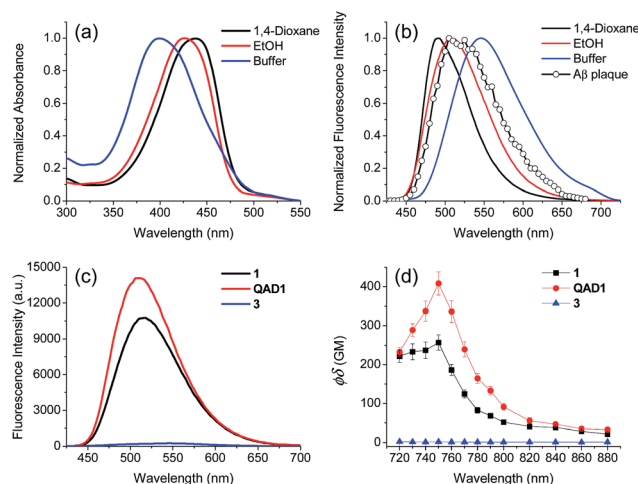
Fig. 1 (a) Normalized absorption and (b) emission spectra of QAD1 ( 1\ \mu\text{M} ) in 1,4-dioxane, EtOH and PBS buffer (10 mM, pH 7.4). Two-photon excited fluorescence (TPEF) spectra (○) acquired from A \beta plaques in a QAD1 -labeled brain slice. (c) Emission spectra of 1 , QAD1 and 3 ( 1\ \mu\text{M} ) acquired in EtOH. (d) Two-photon action spectra of 1 , QAD1 and 3 ( 1\ \mu\text{M} ) acquired in EtOH.
