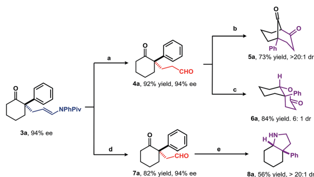
Scheme 3 Synthetic transformations of the product 3a . Reaction conditions: (a) 1 N HCl, Et 2 O, rt, 3 min; (b) (1) 2 N HCl, Et 2 O, rt, overnight; (2) DMP, DCM, rt; (c) SmI 2 , iPrSH, THF, rt; (d) O 3 , Me 2 S, DCM, -78 °C ~ rt; (e) NH 4 OAc, NaBH 3 CN, HOAc, EtOH, rt. DMP = Dess–Martin periodinane.
