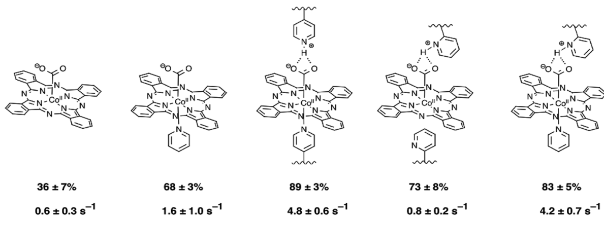
Fig. 7 Proposed activated CO 2 complexes and secondary coordination sphere interaction for each catalyst film studied. Also shown are the faradaic efficiencies and turnover frequencies for each catalyst system determined from CPE measurements.
