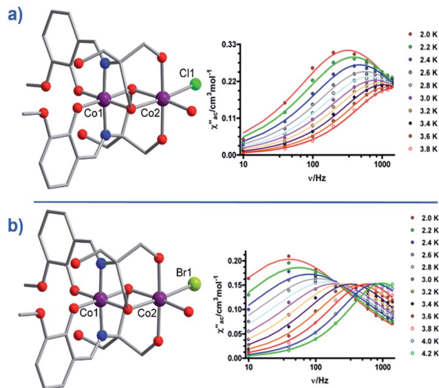
Fig. 15 Molecular structures of [\text{Co}^{\text{III}}\text{Co}^{\text{II}}(\text{LH}_2)_2\text{X}(\text{H}_2\text{O})_4] and the frequency dependence of the out-of-phase magnetic susceptibility collected in a 1000 Oe dc field. (a) \text{X} = \text{Cl} (21) and (b) \text{X} = \text{Br} (22). Colour code: purple (Co), bright green (Cl), light green (Br), blue (N), red (O), grey (C). Hydrogen atoms omitted for clarity. Reprinted with permission from ref. 44. Copyright (2014) American Chemical Society.
