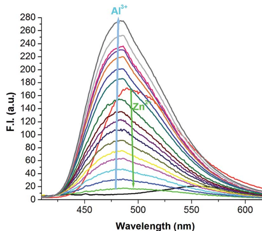
Fig. 5 Selectivity for Al^{3+} over the H_2SAL-NH-Zn^{2+} complex.
