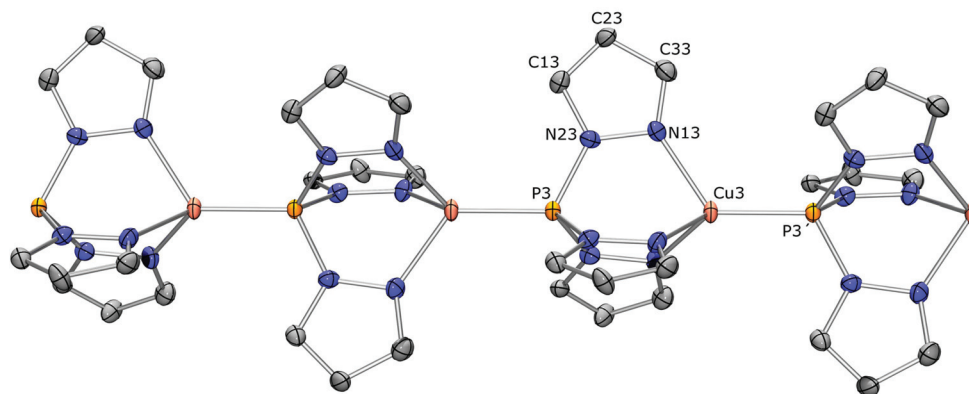
Fig. 7 One-dimensional Cu coordination chain in the crystallographic c -direction of [\text{Cu}^{\text{I}}\text{Cu}^{\text{II}}\text{PF}_6]_n . Only one of the two independent polymers is shown. Location in the unit cell at (0, 0, z ), Wyckoff position a . A slight disorder in this chain has been ignored in the structure refinement. In the drawing, hydrogen atoms, \text{PF}_6 anions and \text{C}_2\text{H}_4\text{Cl}_2 solvent molecules have been omitted for clarity. Symmetry codes: (i) y , x , z − 1/2; (ii) y , x , z + 1/2; (iii) x , y , z + 1. Selected bond lengths [Å] and angles [°]: Cu3–N13 2.034(5), Cu3–P3' 2.081(2), P3–N23 1.700(4), P3...Cu3 3.227(2), N13–Cu3–N13 93.22(17), P3'–Cu3–N13 122.95(12), N23–P3–N23' 101.8(2).
