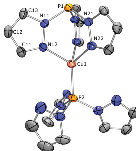
Fig. 5 Displacement ellipsoid plot of [(C^H)_2Cu][PF_6] drawn at the 50% probability level. One of the two independent cations is displayed, PF_6 anions, disordered solvent molecules, and all hydrogen atoms have been omitted for clarity. Selected bond lengths [Å] and angles [°]: Cu1–N12 2.038(3), Cu1–P2 2.0938(11), P1–N11 1.715(4), P1...Cu1 3.3201(12), N12–Cu1–N22 91.25(14), P2–Cu1–N12 123.55(10), N11–P1–N21 99.20(17).
