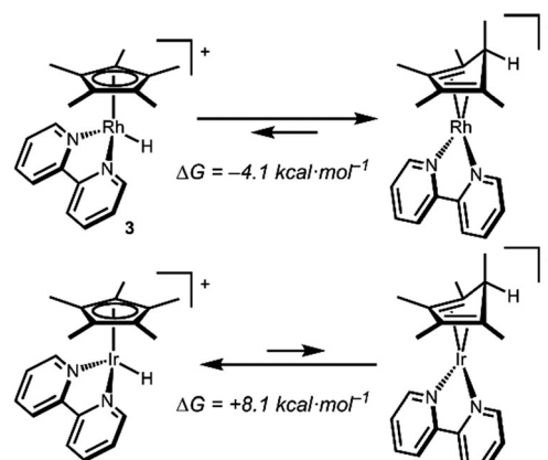
Scheme 3 Free energies for reductive elimination from \text{Cp}^*\text{M}-\text{H} ( \text{M} = \text{Rh}, \text{Ir} ) by DFT.
