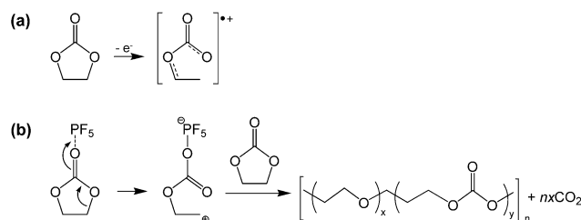
Fig. 11 Possible mechanism for the EC decomposition via strong Lewis acid, PF 5 . Reproduced with permission. 68
