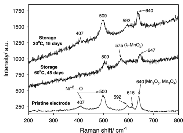
Fig. 10 Ex situ Raman spectra obtained from the pristine LiNi 0.5 Mn 1.5 O 4 , the electrode stored at 30 °C for 15 days, and the electrode stored at 60 °C for 45 days in EC/DMC (1/2)/1.5 M LiPF 6 . Reproduced with permission. 69
