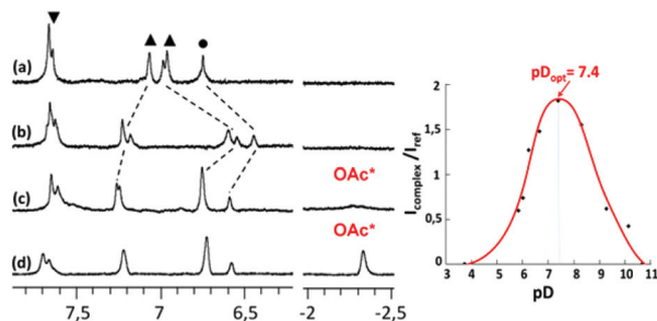
Fig. 2 Left: ^1\text{H} NMR spectra (500 MHz) of free ligand WRim 3 (2.4 mM) in \text{D}_2\text{O} , pD = 8.1 at 300 K (a); in the presence of 1 equiv. of \text{Zn}(\text{NO}_3)_2 in \text{D}_2\text{O} , pD = 7.3 at 300 K (b); ^1\text{H} NMR spectra (500 MHz) of free ligand WRim 3 (2.9 mM) in the presence of 1 equiv. of \text{Zn}(\text{OAc})_2 in \text{H}_2\text{O} , pH = 7.2 at 300 K (c) and at 280 K (d). Right: pD-dependence of the formation of complex [\text{WRim}_3\text{Zn}(\text{OAc})]^+ in \text{D}_2\text{O} (2.5 mM). (▼) HAR. "down"; (▲) HIm; (●) HAR. "up".
