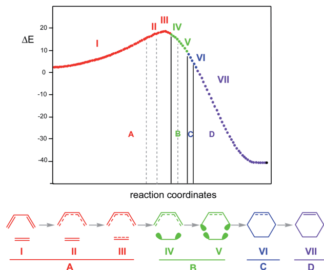
Fig. 6 Reaction path calculated by means of the IRC method for the DA reaction between butadiene 1 and ethylene 2 . \Delta E are in \text{kcal mol}^{-1} . A bonding between atoms in all phases is demonstrated by the standard Lewis representation; however, in the case of phases IV and V, ellipses reflect the non-bonding electron density concentrated in the C atoms. The four colours represent the four main groups in which the bonding changes can be categorised.
