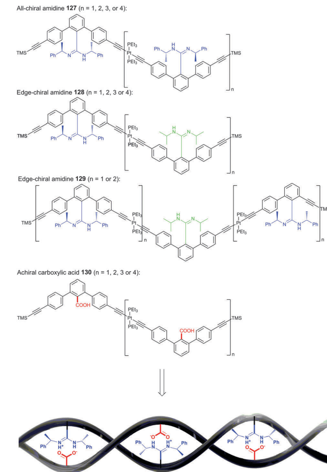
Scheme 14 Overview of the various amidine and carboxylic acid strands by Yashima and co-workers and their double helix formation.
