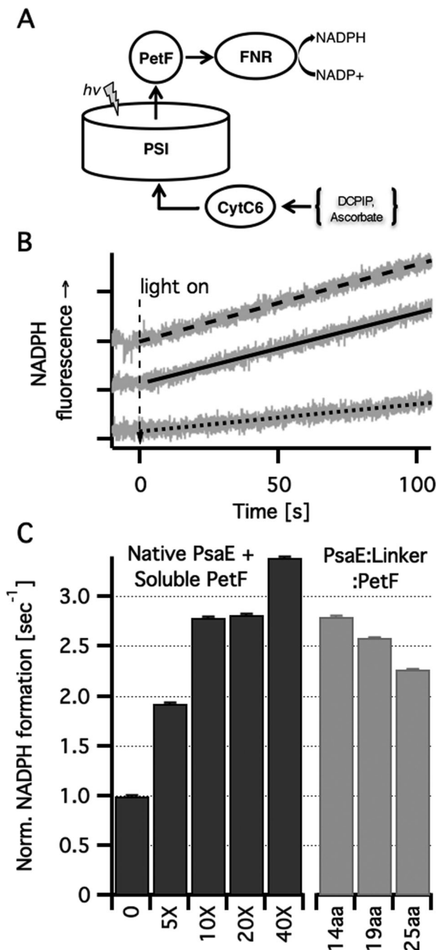
Fig. 4 In vitro light dependent \text{NADP}^+ reduction. (A) Scheme of the electron transport chain in solution. Photoexcited PSI was used to reduce PetF that carried the electrons to FNR where they were used for \text{NADP}^+ reduction to NADPH. Ascorbic acid was used as a sacrificial electron donor by reducing (via DCPIP) CytC6 that transferred the electrons to the oxidizing end of PSI. (B) NADPH formation rates were measured in vitro by monitoring the linear increase in NADPH fluorescence. Typical traces (grey lines) and their linear fits are shown for PSI with no PetF (dotted line), PSI with ten-fold PetF molar excess (dashed line) and PSI reconstituted with PsaE:19aa:PetF (solid line). (C) NADPH formation rates normalized by the rate for PSI reconstituted with native PsaE without PetF. Molar excess of soluble PetF to PSI are indicated. No PetF was added to the PSI complexes reconstituted with PsaE::PetF fusion proteins.
