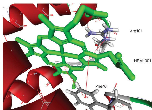
Fig. 2 Details of \pi - \pi and cation- \pi interactions for the HEM1001 of hemoglobin from midge larva Propislocerus akamusi (PDB ID code 1x3k). The interactions are marked with red lines ( \pi - \pi interactions: HEM1001:C—Phe46, HEM1001:D—Phe46; cation- \pi interactions: HEM1001:D—Arg101:NE).
