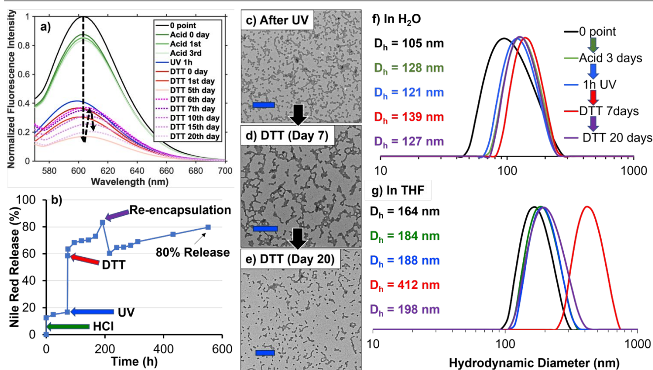
Figure 7. Stimuli-triggered Nile Red release from worm-like TORC-NGs upon sequential addition of HCl (acidification to pH=4 for 3 days) followed by 1 h irradiation with 254 nm UV light, addition of 51.1 mM DTT and incubation for 20 days as monitored by fluorescence spectroscopy (a, b). This revealed, at day 5+, sudden re-encapsulation of Nile Red induced by morphological transitions from short to long worm-like nanostructures followed by the slower breakdown of long worms to short worms over the next 15 days as evidenced by TEM (c – e; scale bars = 500 nm). DLS was also conducted to track the sizes of worm-like TORC-NGs after adding different stimuli in H 2 O (f) and THF (g).
