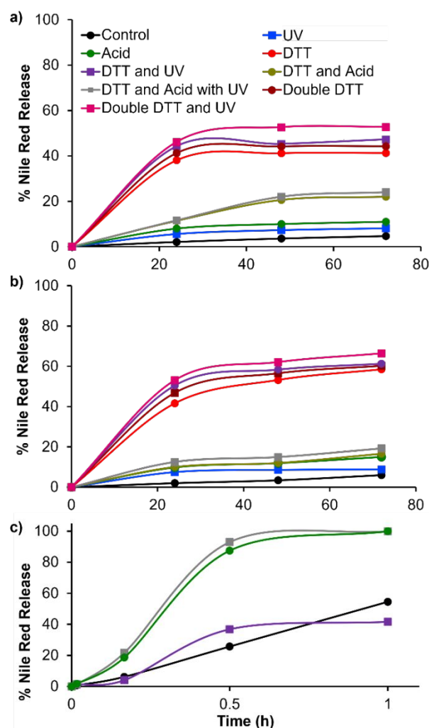
Figure 4. Nile red release profiles for spherical TORC-NGs (a), worm-like TORC-NGs (b) and non-CCL nanosphere (c) upon application of various stimuli simultaneously (Legend applies to all plots; control = no stimuli; acid = adjusted to pH 4 with HCl/H 2 O; DTT = addition of 66.2 mM DTT for spherical TORC-NG and 51.1 mM DTT for worm-like TORC-NG; UV = 1 h irradiation with 254 nm UV light).
