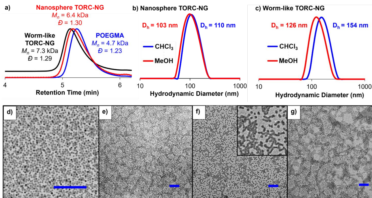
Figure 2. PhotoATR-PISA fabrication of TORC-NGs with target \text{DP}(\text{PGMA}) = 86 for nanosphere and \text{DP}(\text{PGMA}) = 129 for worm-like showing clear shifts in the retention time via GPC (a). DLS of nanosphere (b) and worm-like (c) TORC-NGs provided evidence of TORC-CCL stabilization showing intact polymeric particles with larger hydrodynamic diameter when transferred to good solvent (i.e., chloroform) and compared to selective solvent (i.e., MeOH). This is confirmed via TEM of nanosphere (d, e) and worm-like (f, g) TORC-NGs cast onto grids from MeOH and \text{CHCl}_3 , respectively (Scale bars = 500 nm).
