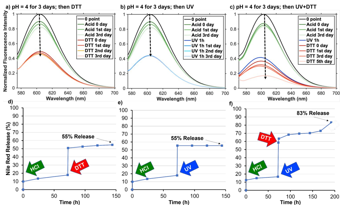
Figure 5. Fluorescence spectra of Nile Red loaded, worm-like TORC-NGs after acidification to pH = 4 with HCl and incubating for 3 days followed by addition of DTT alone ( c = 51.1 M; a, d), irradiation with 254 nm UV light for 1 h alone (b, e), or introduction of UV light and DTT sequentially (c, f) leading to AND-gate cargo release only when both stimuli were applied.
