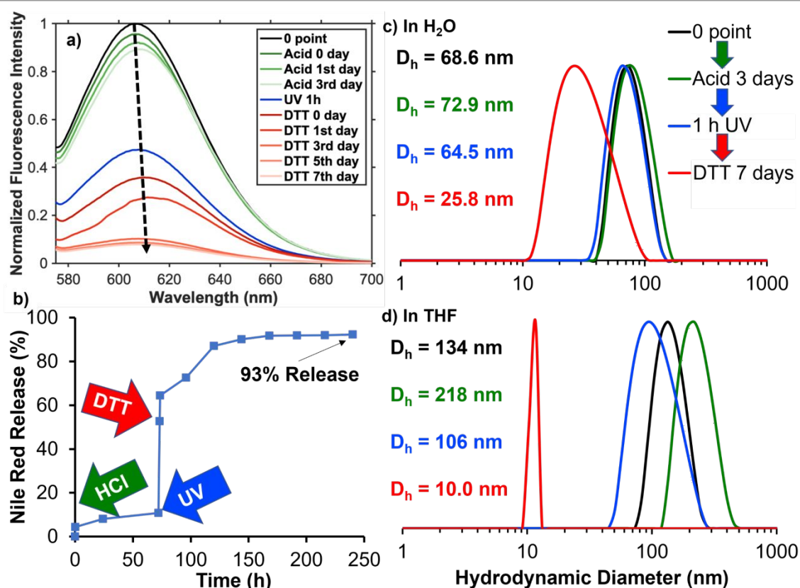
Figure 6. Stimuli-triggered Nile Red release from nanosphere TORC-NGs upon sequential addition of HCl (acidification to pH=4 for 3 days) followed by 1h irradiation with 254 nm UV light, subsequent addition of 66.2 mM DTT and incubation for 7 days as monitored by fluorescence spectroscopy (a, b). DLS was also conducted to track the sizes of nanosphere TORC-NGs after adding different stimuli in H 2 O (c) and THF (d).
