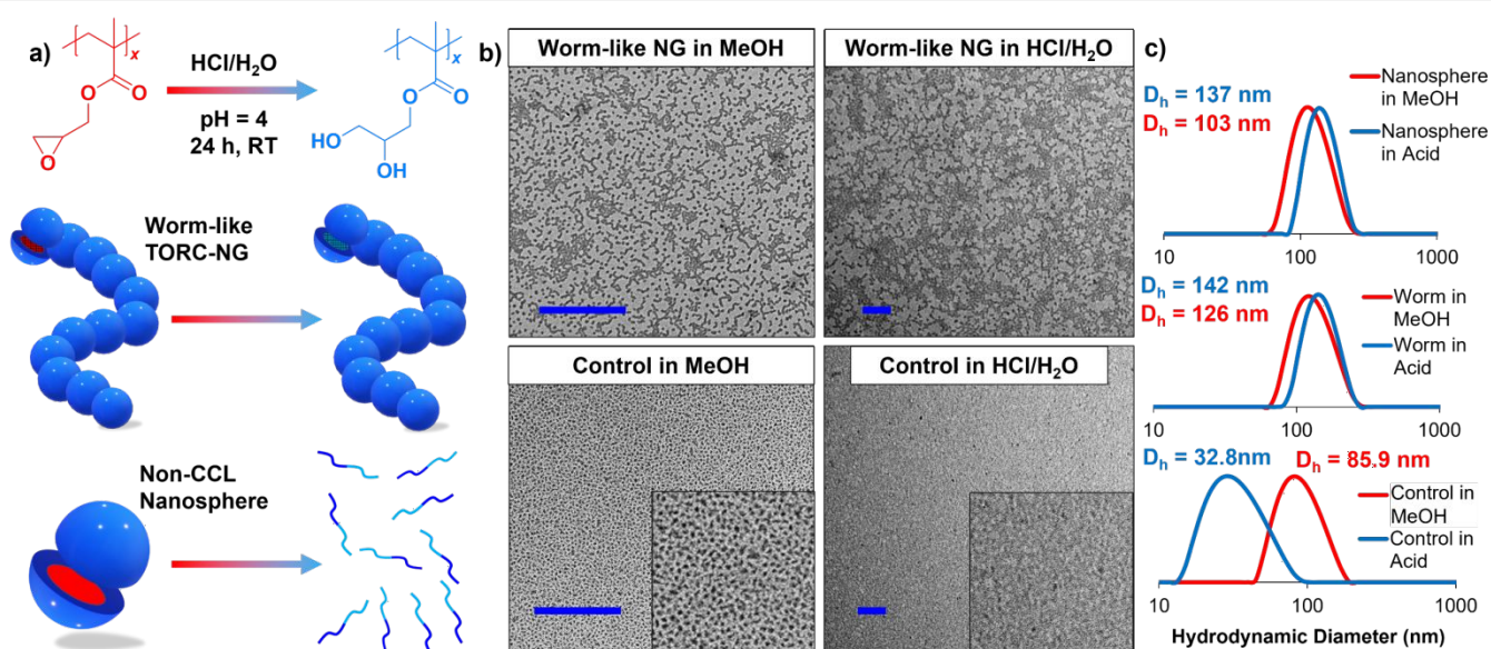
Figure 3. Acid-catalysed hydrolysis of PGMA pendant epoxide rings in \text{HCl}/\text{H}_2\text{O} ( \text{pH} = 4 ) which causes TORC-NGs to swell and non-CCL nanospheres to fully disassemble (a). This is confirmed via TEM of worm-like TORC-NGs and non-CCL nanosphere controls in MeOH and after reacting in \text{HCl}/\text{H}_2\text{O} for 24 h (b; Scale bars = 500 nm; insets = 500 x 500 nm). This is confirmed via DLS through observed swelling of D_h after hydrolysis for TORC-NGs and decreases in D_h for non-CCL nanospheres due to disassembly (c).
