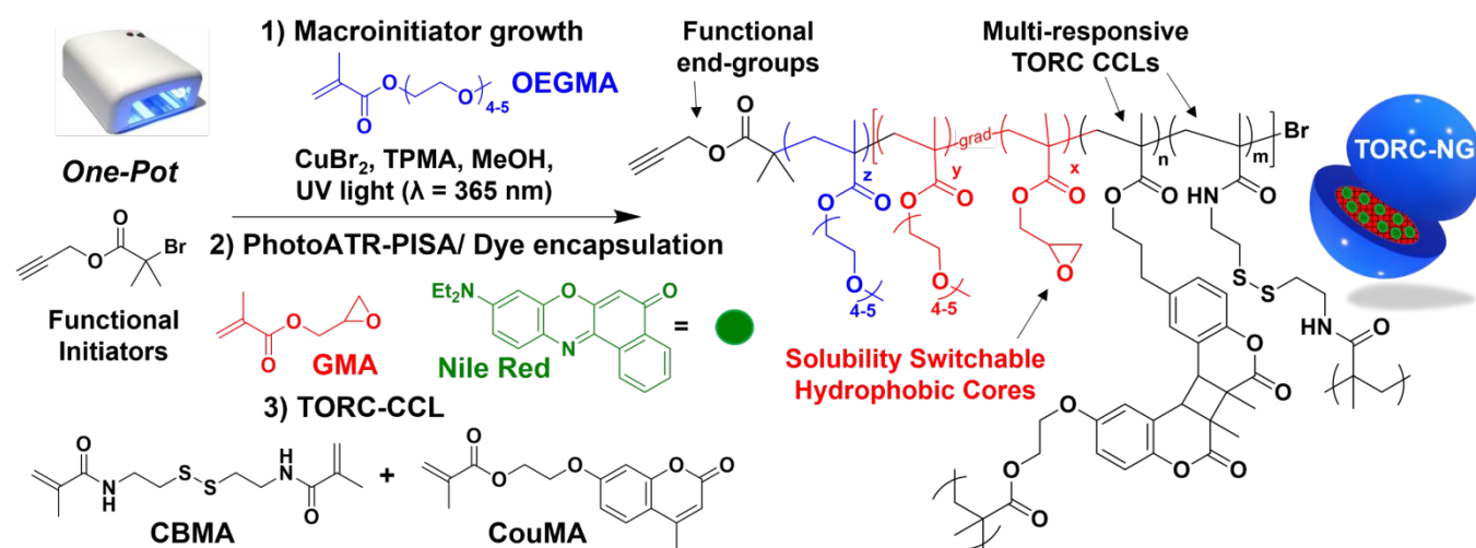
Scheme 1. Synthesis of Nile Red encapsulated, light/redox/acid-responsive gradient copolymer TORC-NG via one-pot, PhotoATR-PISA using redox-responsive CBMA crosslinker with disulfide bonds, UV-responsive CouMA crosslinkers and pH sensitive, PGMA hydrophobic cores.
