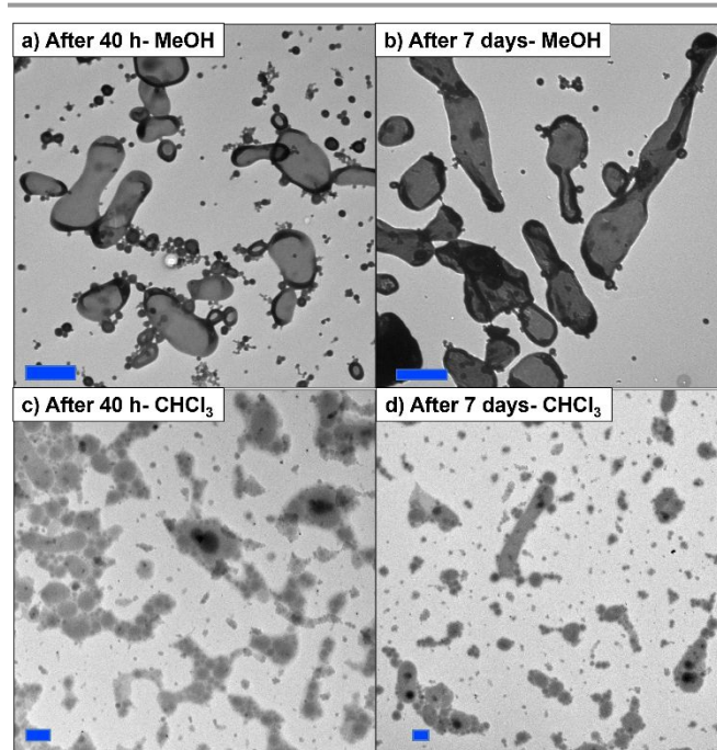
Figure 8. TEM images of PBMA- b -POEGMA vesicle TORC-NGs as conversion of CBMA increases showing large, elliptical polymersomes at low conversions (a) that transition to large, multi-micron long tubesome structures at full CBMA conversion (b). The stability of these materials at both stages is confirmed upon solvent switch to \text{CHCl}_3 and imaging using TEM (c, d; all scale bars = 2.0 \mu\text{m} ).
