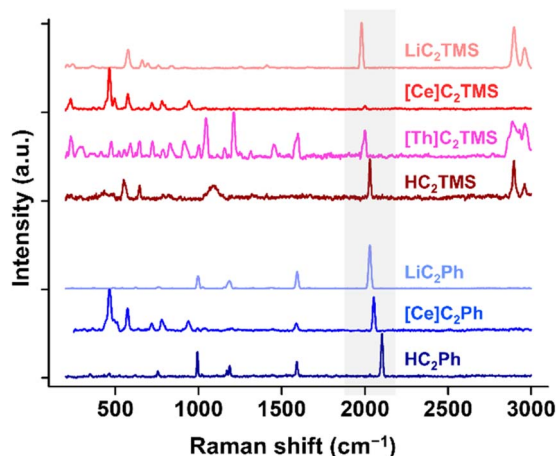
Fig. 6 Raman spectra of 1-Ce TMS , 1-Ce Ph , and 1-Th TMS , and comparison with a lithium-acetylide complex and protonated alkyne.
