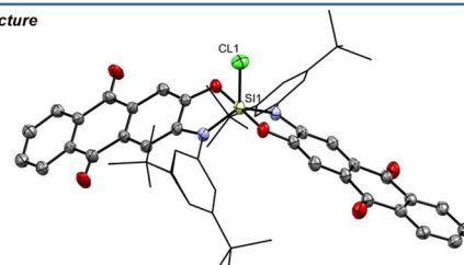
Fig. 5 (a) Synthesis of pentacoordinate silicon complexes with neutral and anionic donors. (b) Molecular structure of [1-Cl][PPh 4 ] determined by SCXRD analysis. Hydrogen atoms and the \text{PPh}_4 cation are omitted for clarity. Thermal displacement ellipsoids are displayed at the 50% probability level. Selected bond lengths [pm]: Si1–Cl1: 211.64(10), Si1–O1: 174.78(18), Si1–N1: 178.1(2). Selected bond angles [°]: N1–Si1–N1: 128.16(10), O1–Si1–O4: 177.74(9), N1–Si1–Cl1: 116.45(8), O1–Si1–Cl1: 91.53(7).
