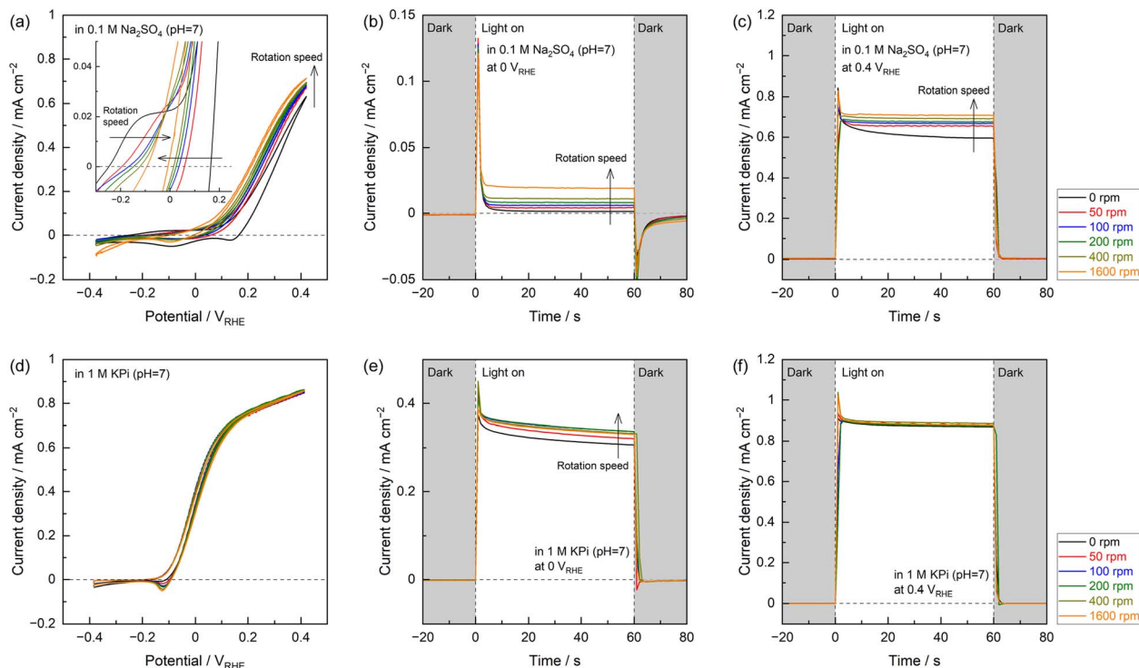
Fig. 2 (a) CV data and current–time curves acquired at applied potentials of (b) 0 and (c) 0.4 V RHE with a rotating Nb:STO disk electrode at various rotation rates in a 0.1 M Na 2 SO 4 electrolyte and (d–f) the same plots obtained in a 1 M KPi electrolyte. A 365 nm LED light source was used.
