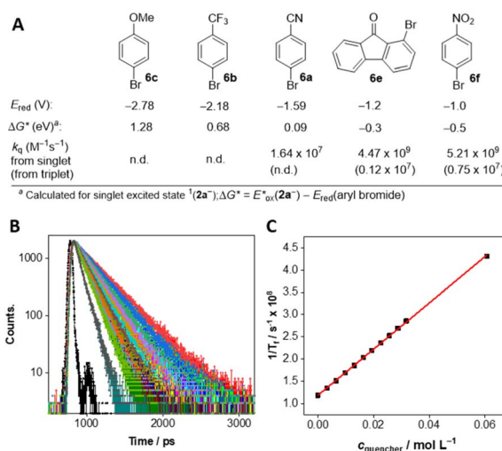
Fig. 7 (A) Quenching rate constants (in units of \text{M}^{-1} \text{s}^{-1} ) for 2a - in the singlet or triplet excited state by bromoarenes and the corresponding thermodynamic data for electron transfer from 2a - in the singlet excited state. For references on reduction potentials, see text. Fluorescence lifetime quenching of 2a - with 6f ; (B) fluorescence decays of 2a - at different concentration of 6f and (C) the corresponding Stern–Volmer plot.
