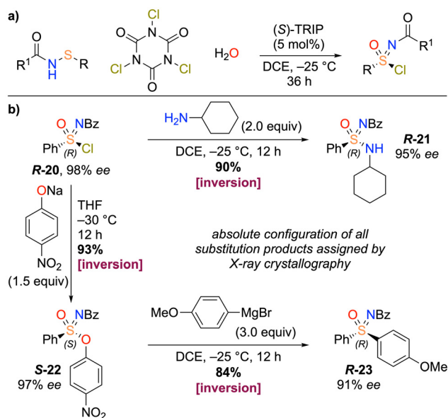
Scheme 5 (a) Enantioselective hydrolysis to access enantio-enriched sulfonylimidates; (b) S(vi) substitution reactions with sulfonylimidoyl chloride R-20 to generate enantio-enriched sulfonylimidamide R-21 , sulfonylimidate S-22 , and sulfoximine R-23 .
