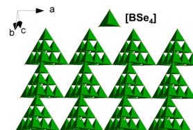
Fig. 9 The layer in the structure of \text{Li}_{6-x}\text{Cs}_x\text{B}_{10}\text{Se}_{18} ( x \approx 1 ).
