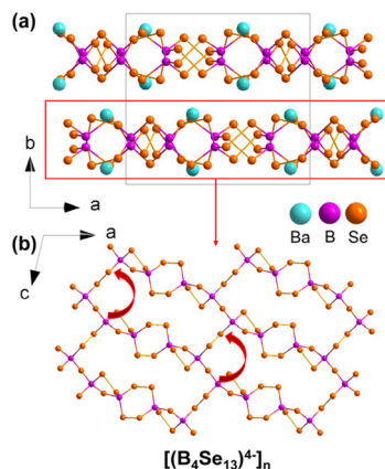
Fig. 7 The structures of (a) the \text{Ba}_2\text{B}_4\text{Se}_{13} layer and (b) the [(\text{B}_4\text{Se}_{13})^{4-}]_n layer.
