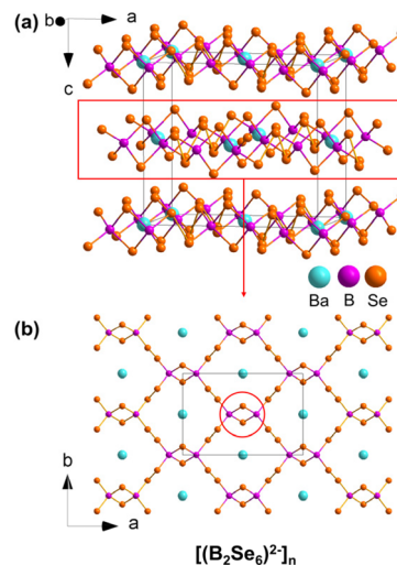
Fig. 8 The structures of (a) the \text{BaB}_2\text{Se}_6 layer and (b) the [(\text{B}_2\text{Se}_6)^{2-}]_n layer.
