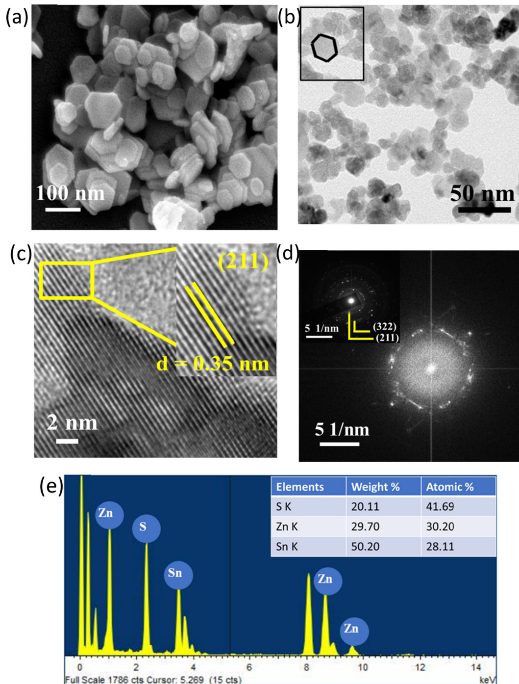
Fig. 2 (a) FE-SEM image, (b) low-resolution TEM image, (c) HR-TEM image and the interplanar spacing corresponding to the (211) plane (inset), (d) FFT and SAED pattern (inset), (e) energy dispersive X-ray spectrum and spectroscopic analysis (EDX) for ZTS NCs.
