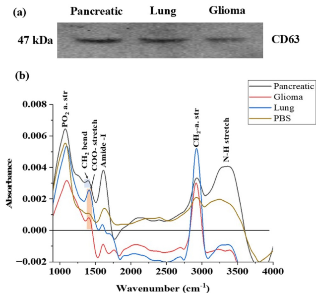
Fig. 3 (a) Western blot analysis of the common tetrapanin cell surface exosomal marker CD63; (b) ATR-FTIR spectra of exosomes originated from pancreatic, glioma and lung cancer cells.
