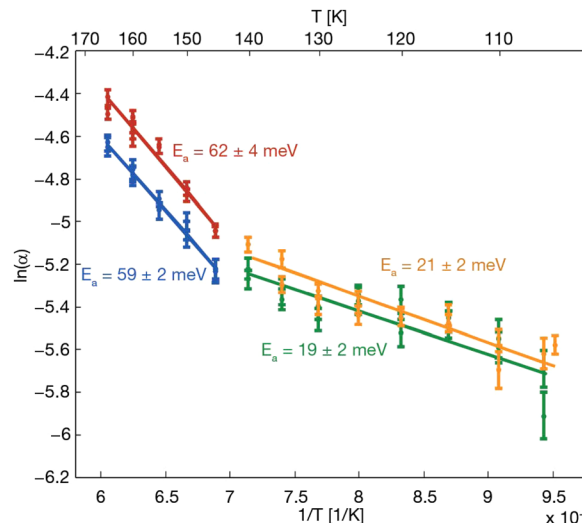
Fig. 11 The Arrhenius plot from temperature-dependent measurements of \text{C}_4\text{H}_4\text{S} dynamics on \text{Cu}(111) , taken at 0.7 \text{ \AA}^{-1} along the \overline{\Gamma\text{K}} -azimuth, reveals two competing activated processes. The gradient gives an apparent activation barrier for rotation of 19 \pm 2 \text{ meV} at 0.015 \text{ ML} (green) and 21 \pm 2 \text{ meV} at 0.022 \text{ ML} (orange), while jump diffusion is more strongly activated with E_a = 59 \pm 2 \text{ meV} at 0.015 \text{ ML} (blue) and E_a = 62 \pm 4 \text{ meV} at 0.022 \text{ ML} (red). (Reprinted with permission from ref. 66, Copyright 2013 by the American Chemical Society).
