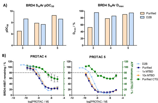
Fig. 3 A) Correlation between crude and purified samples; B) curves from HiBiT and CTG assays for D2B samples ( N = 1), purified samples ( N = 2), and spiking experiments of purified PROTAC with MTBD ( N = 2). Error bars represent SEM.
