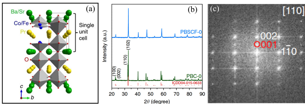
Fig. 14 Structural and morphological characterization of \text{PrBaCo}_2\text{O}_{5+\delta} (PBC) and \text{PrBa}_{0.5}\text{Sr}_{0.5}\text{Co}_{1.5}\text{Fe}_{0.5}\text{O}_{5+\delta} (PBSCF) DP oxides. (a) Schematic of the PBC/PBSCF DP crystal structure, (b) XRD patterns of PBC and PBSCF powders. (c) Fast Fourier transform (FFT) pattern (obtained from the region of \sim 23 \text{ nm} \times 23 \text{ nm} ) 101 copyright 2017, Springer Nature.
