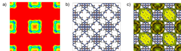
Fig. 3 a) 2D representation of the benzene presence density in ZIF-8_Br. b) Illustration of 2 \times 2 supercell of ZIF-8_Br structure and c) 3D representation of the benzene presence density in ZIF-8_Br.
