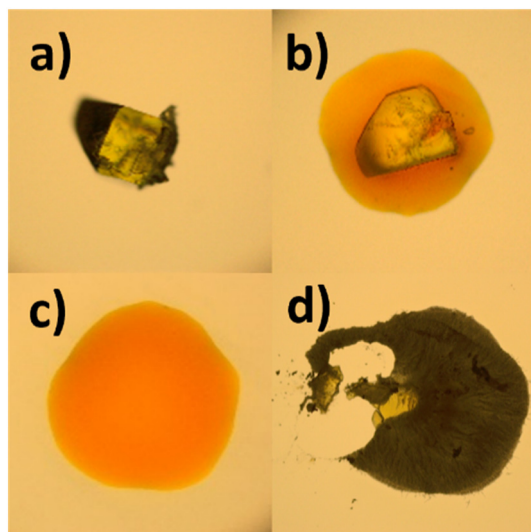
Fig. 4 Crystal of AlZ 1a a) before and b) shortly after irradiation with UV-light ( \lambda = 365 nm, 1 min) showing a partial UV-induced phase transition, c) fully liquefied after further irradiation with UV-light ( \lambda = 365 nm, 1 min) and d) after recrystallization through irradiation with green light ( \lambda = 520 nm, 5 min).
