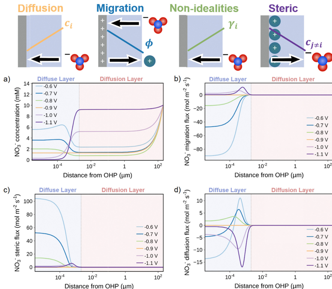
Fig. 3 (a) Simulated concentration profiles for NO 3 - function of distance from the outer Helmholtz plane (OHP) at applied potentials ranging from -0.6 to -1.1 V vs. SHE. NO 3 - fluxes corresponding to (b) migration, (c) steric effects, and (d) diffusion as a function of distance from the OHP at applied potentials ranging from -0.6 to -1.1 V vs. SHE. Negative and positive fluxes indicate directionality towards the electrode and away from the electrode, respectively. The dashed line at 2 nm indicates the approximate boundary between the diffuse and diffusion layers ( i.e. , the distance from the OHP at which the electrolyte transitions from electrically-charged to electrically-neutral).
