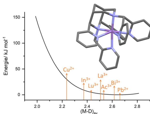
Fig. 3 Exemplary hole-size curve calculated for the heptadentate ligand L 6 (see Scheme 3 below). Arrows depict the approx. metal ion size ( i.e. , the average metal-donor distance for the appropriate metal ion – ligand combination) for a range of metal ions relevant for radiopharmaceutical applications. 16,22,42,55
